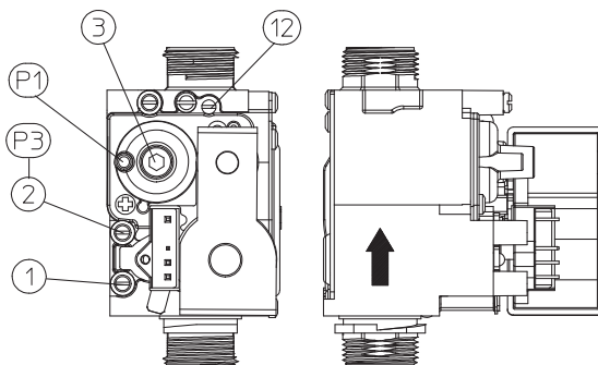
Valvola Gas SIT 848
